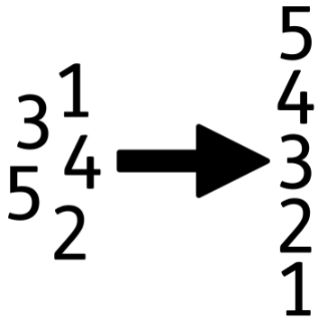
sequence
