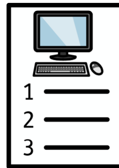
algorithm
