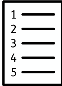
steps
