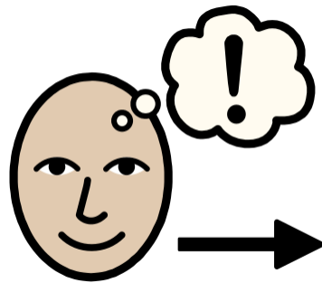
predict
